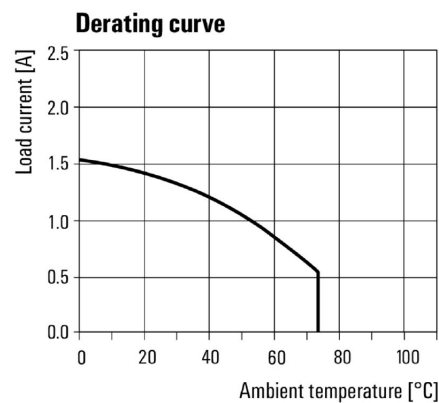
Deratingkurve
