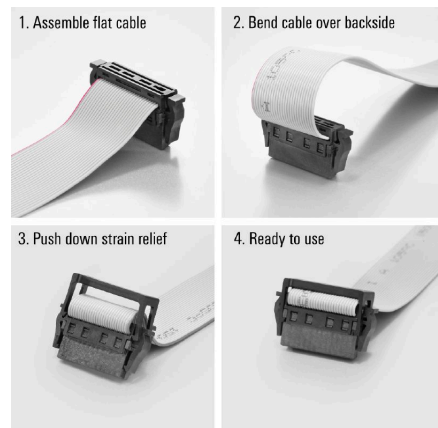
Assembly of strain relief
