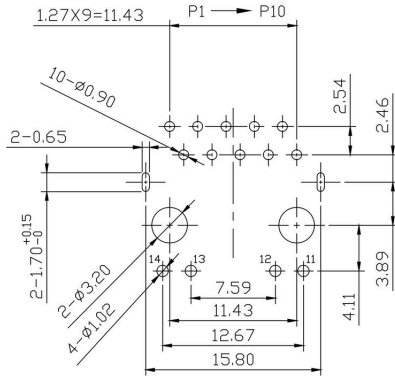
PCB LAYOUT 2
