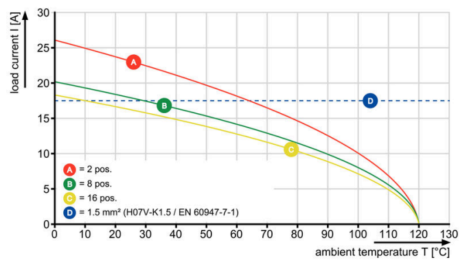
BCZ 3.81../90 & /270 - SC-SMT 3.81../135
