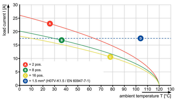
BCZ 3.81../90 & /270 - SC 3.81../135
