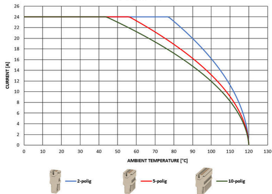
Derating APG 2.5...
