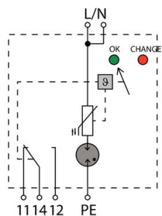
Principle circuit diagram
