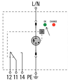
Schematic circuit diagram
