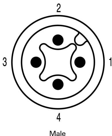
Male
