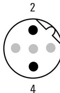
Pin
