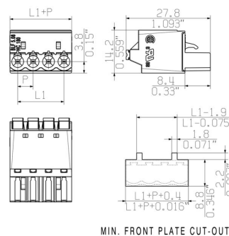
MIN. FRONT PLATE CUT-OUT
