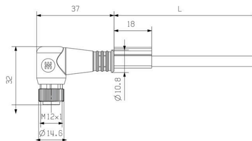
Angled socket
