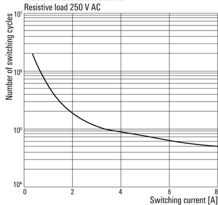
Electrical Endurance at AC
