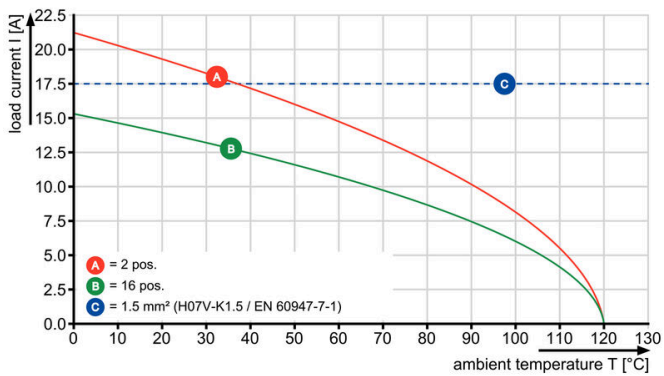
BCZ 3.81/12/180 - SC-SMT 3.81/12/180
