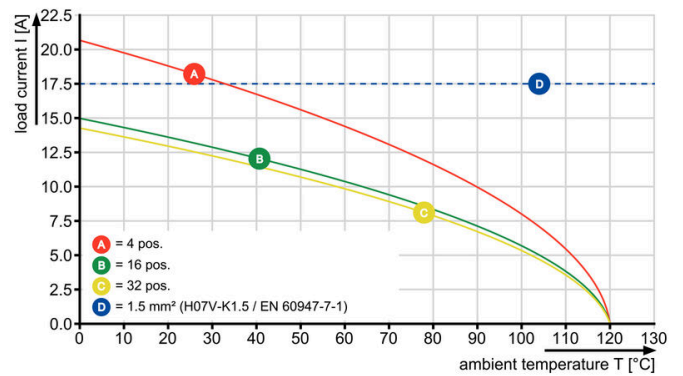
BCZ 3.81/12/180 - SCD-THR 3.81/12/180
