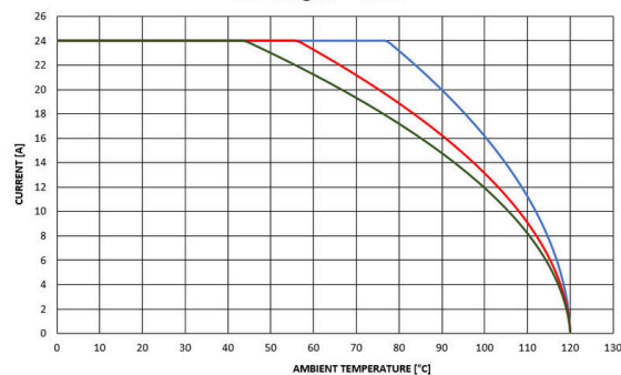
Derating APG 2.5...
