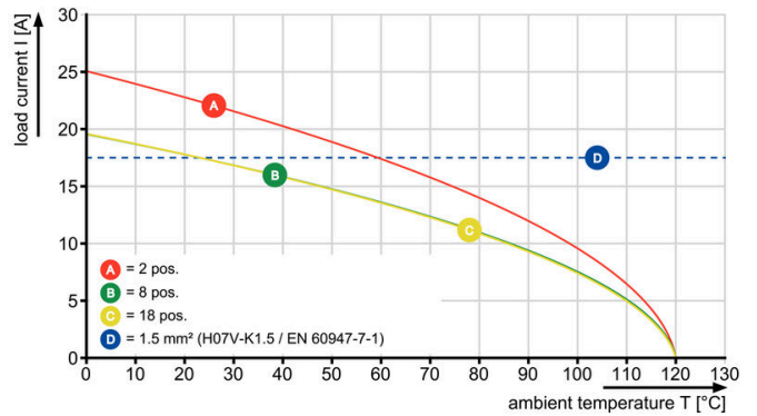
BCF 3.81/11/180 - SC 3.81/11/90
