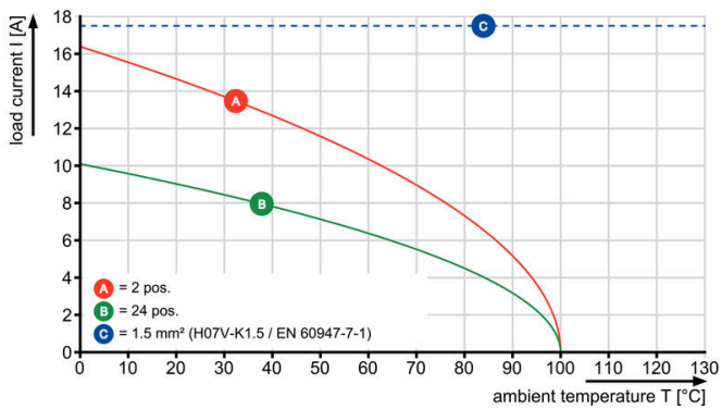
BL 3.50/15/180 - SL-SMT 3.50/15/90
