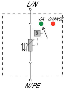
Schematic circuit diagram
