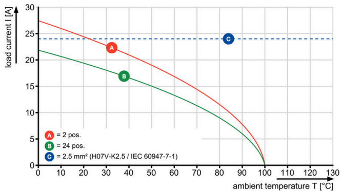
BLF 5.08HC/./270 - SL 5.08HC/./90
