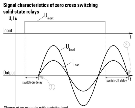
Shown at an example with resistive load. 1. Switches on at first zero cross of mains voltage while control input gets signal. 2. Switches off at next zero cross of mains current after control input signal was switched off. Switching DC voltages is not possible with this solid-state relays.
