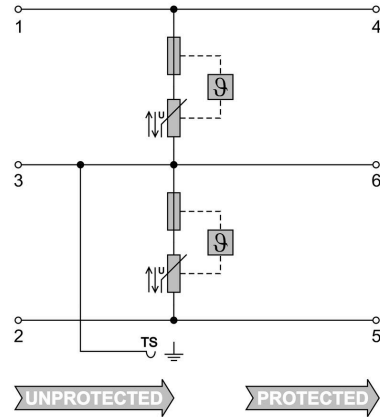
Circuit diagram
