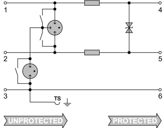
Circuit diagram
