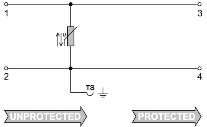
Circuit diagram
