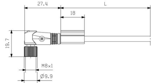
Angled socket
