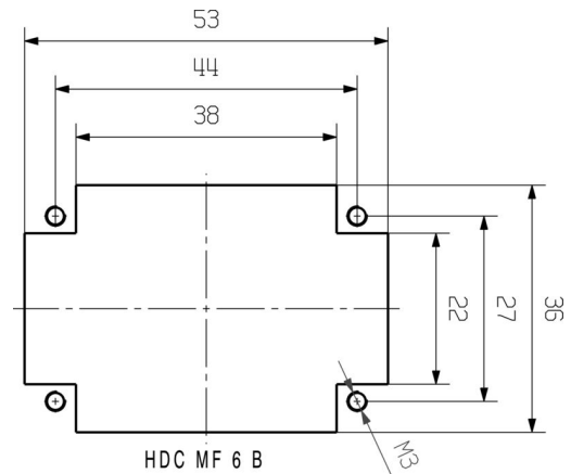
mounting cutout
