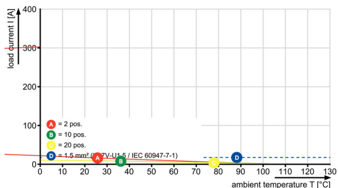
CPS 3.81/./90 - CH 3.81/./90G
