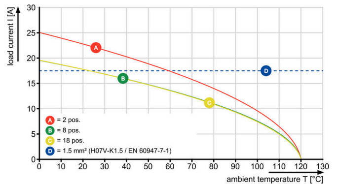
BCF 3.81/15/180 - SC 3.81/15/180
