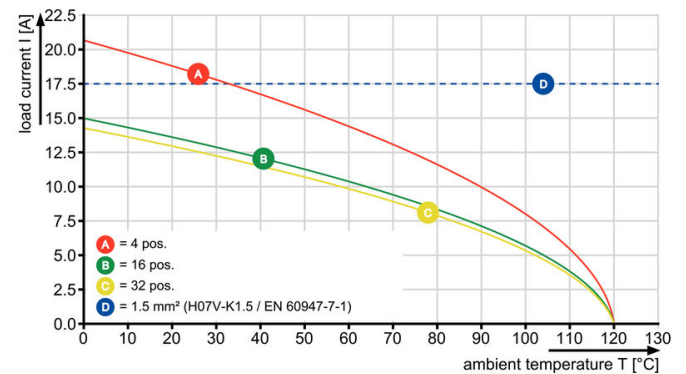
BCZ 3.81/./180 - SCD-THR 3.81/./90
