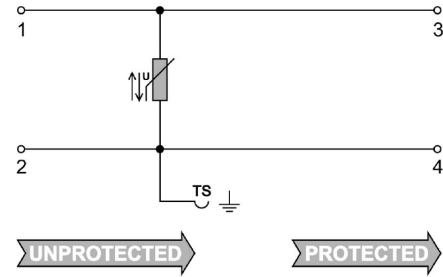
Circuit diagram
