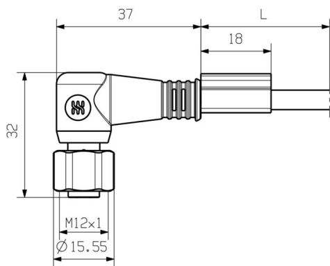
Angled socket
