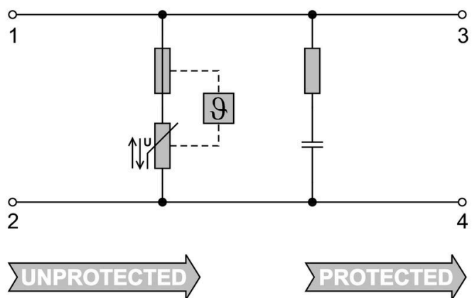
Circuit diagram
