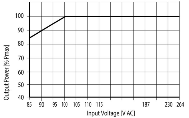
AC-Input Derating
