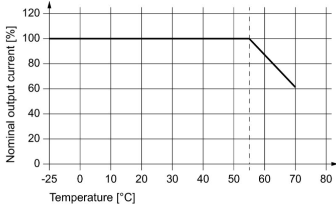
Temperature Derating
