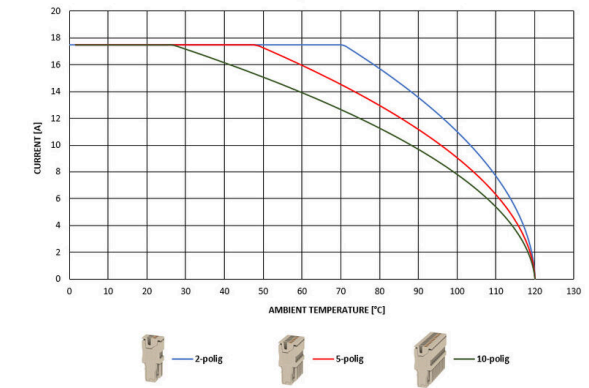
Derating APG 1.5...
