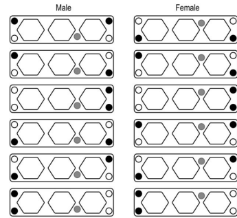
Coding scheme
