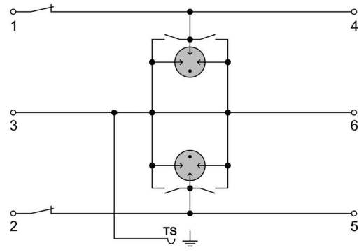
Circuit diagram
