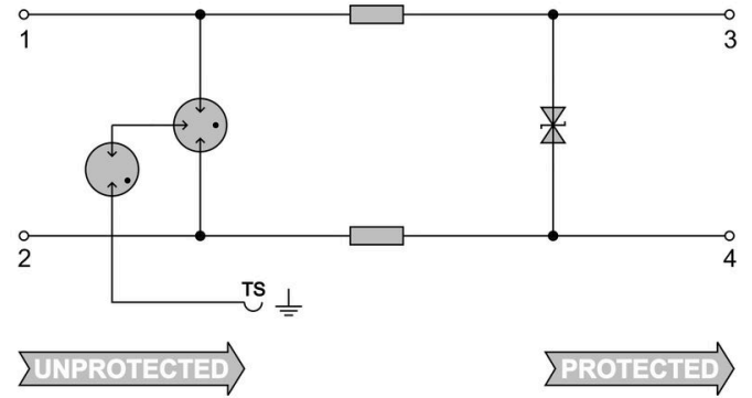
Circuit diagram
