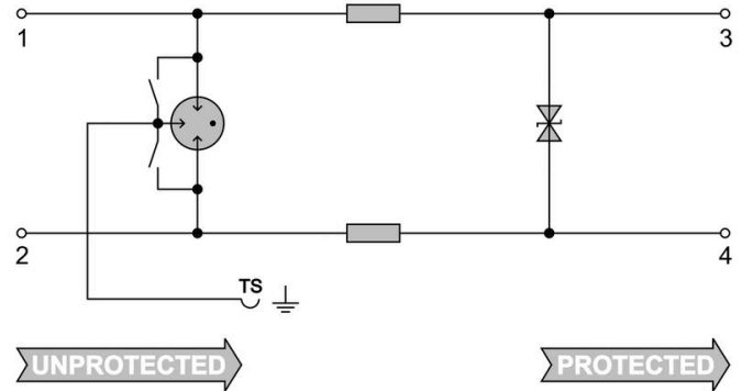
Circuit diagram
