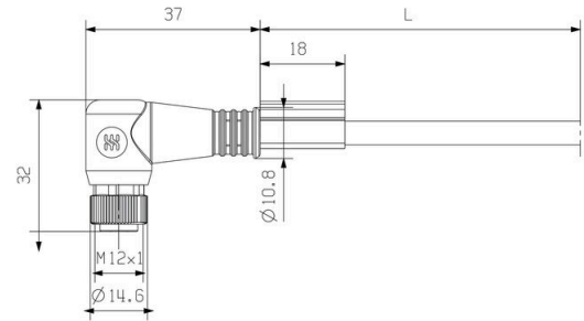
Angled socket
