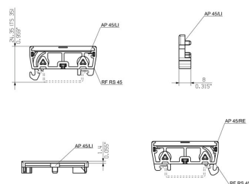
RAIL MOUNTING
