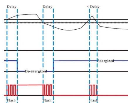
over mode working timing diagram
