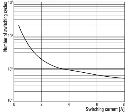
Electrical Endurance at AC
