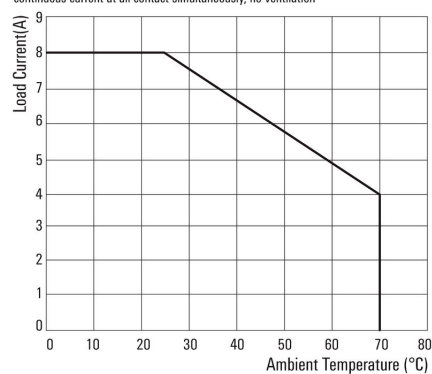
Derating Curve
