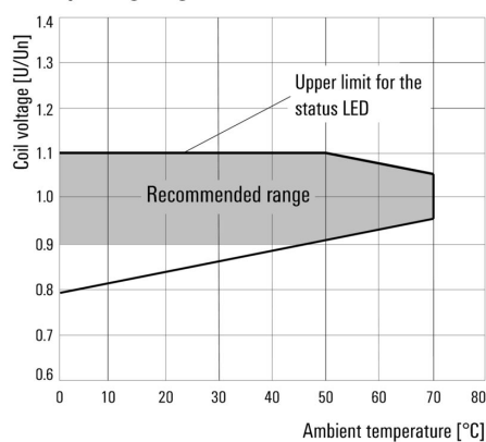
Coil Operating Range AC
