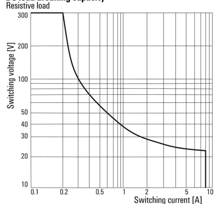
DC load breaking capacity
