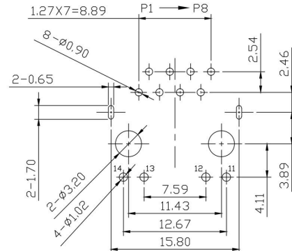
PCB LAYOUT 2
