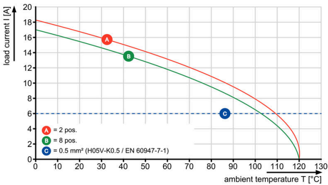
LSF-SMT 7.50/./135 3.5
