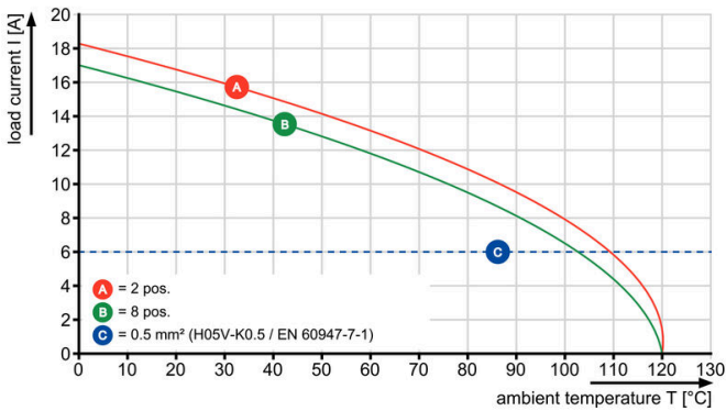
LSF-SMT 7.50/./135 1.5
