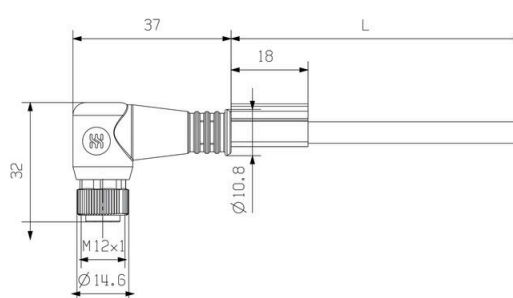
Angled socket
