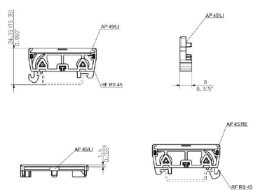
RAIL MOUNTING
