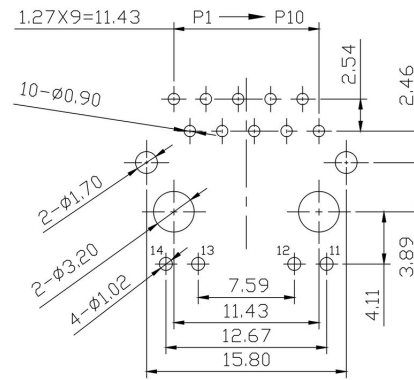
PCB LAYOUT 1
