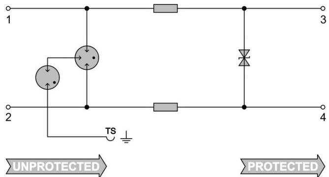
Circuit diagram
