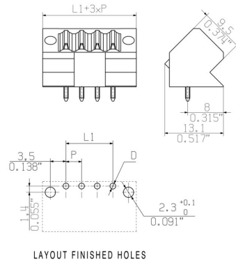
LAYOUT FINISHED HOLES
