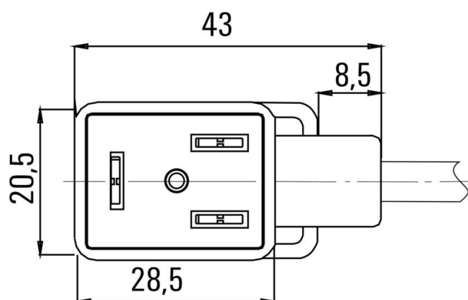
Pole scheme
