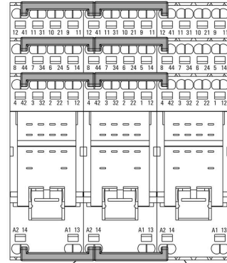
Cross connection: SCM-I QV P Part-No. 8870850000 Sockets: SCM-I xCO P
